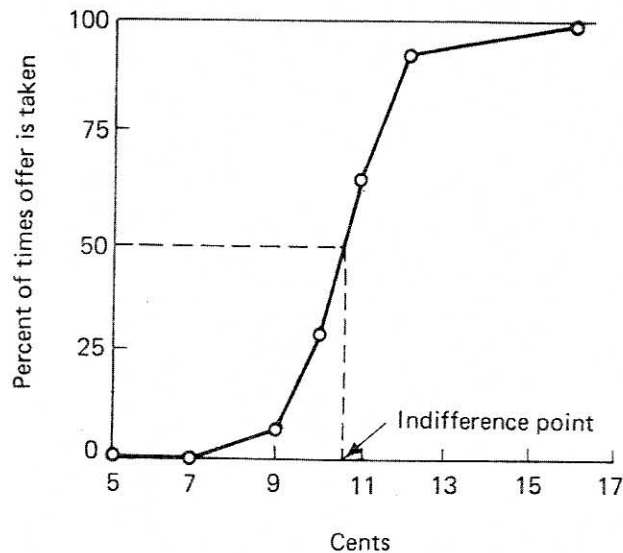
Fig. 5.8 Proportion of times an offered gamble was accepted by one of the subjects in the Mosteller and Nogee experiment.
