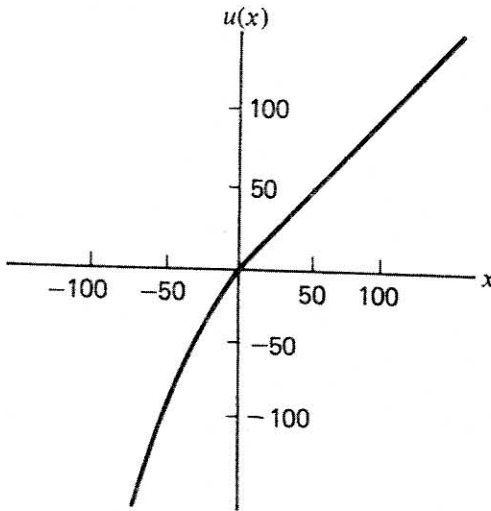
Fig. 5.12 Utility function for a typical subject.
