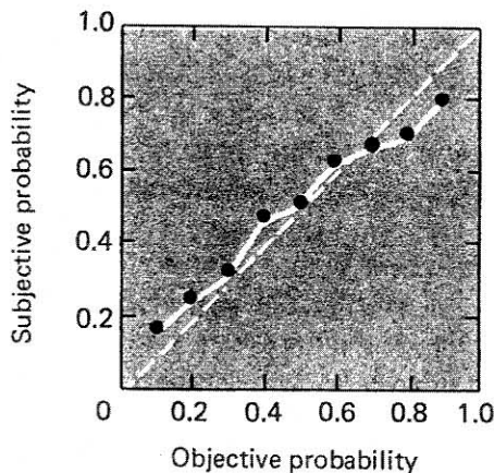
Fig. 5.13 Subjective probability function for a typical subject.
